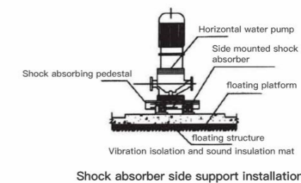
Shock absorber side support installation
