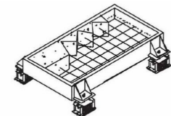
Side support type (IBF-B type)
